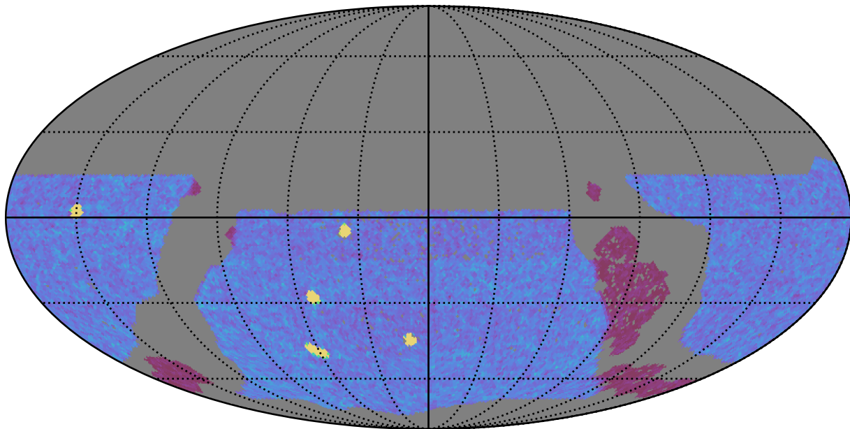
too_combined_s0.8_v3.4_10yrs WFD y band: NVisits
