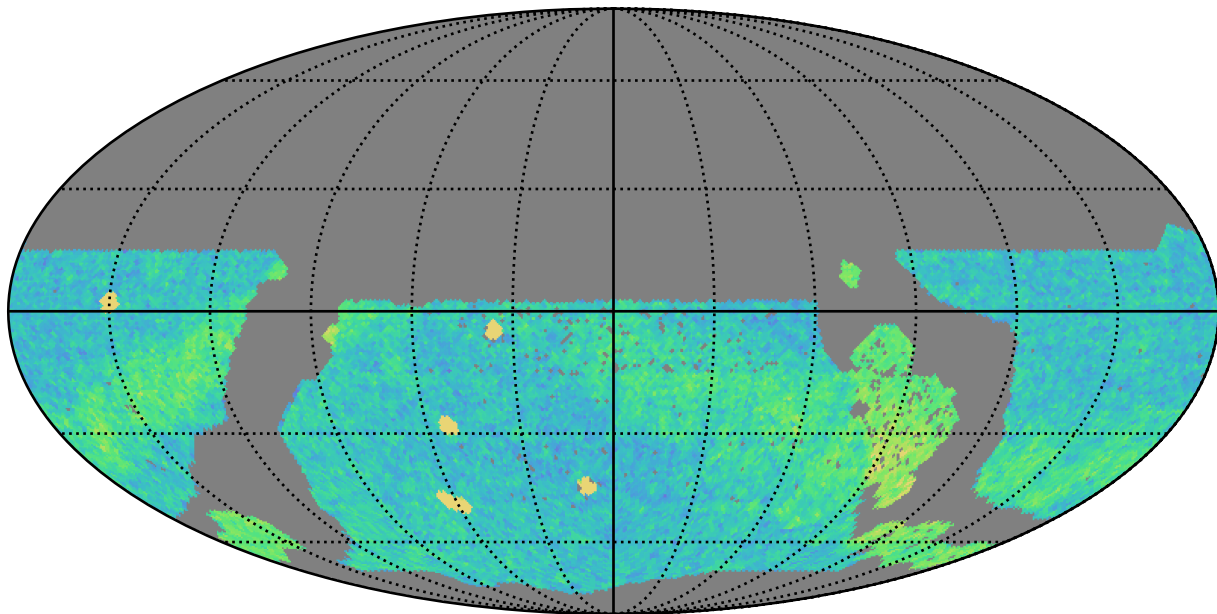
too_combined_s0.8_v3.4_10yrs WFD r band: NVisits
