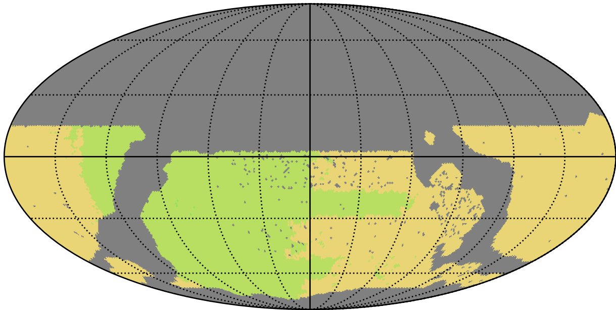
too_combined_s0.8_v3.4_10yrs WFD all bands: NSeasons
