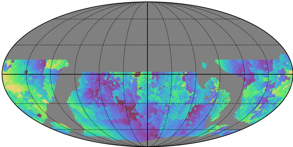
too_combined_s0.8_v3.4_10yrs WFD u band: Min solarElong
