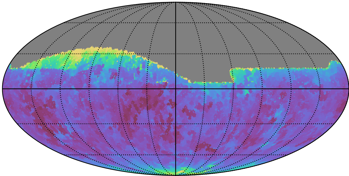
too_combined_s0.8_v3.4_10yrs Yr 1 all bands: Min seeingGeom
