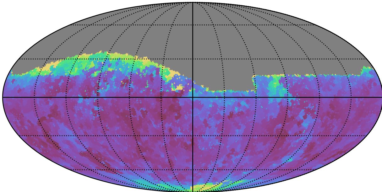
too_combined_s0.8_v3.4_10yrs Yr 1 r band: Min seeingEff
