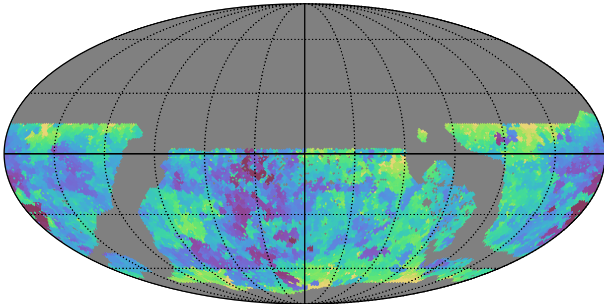
too_combined_s0.8_v3.4_10yrs WFD g band: Min seeingEff
