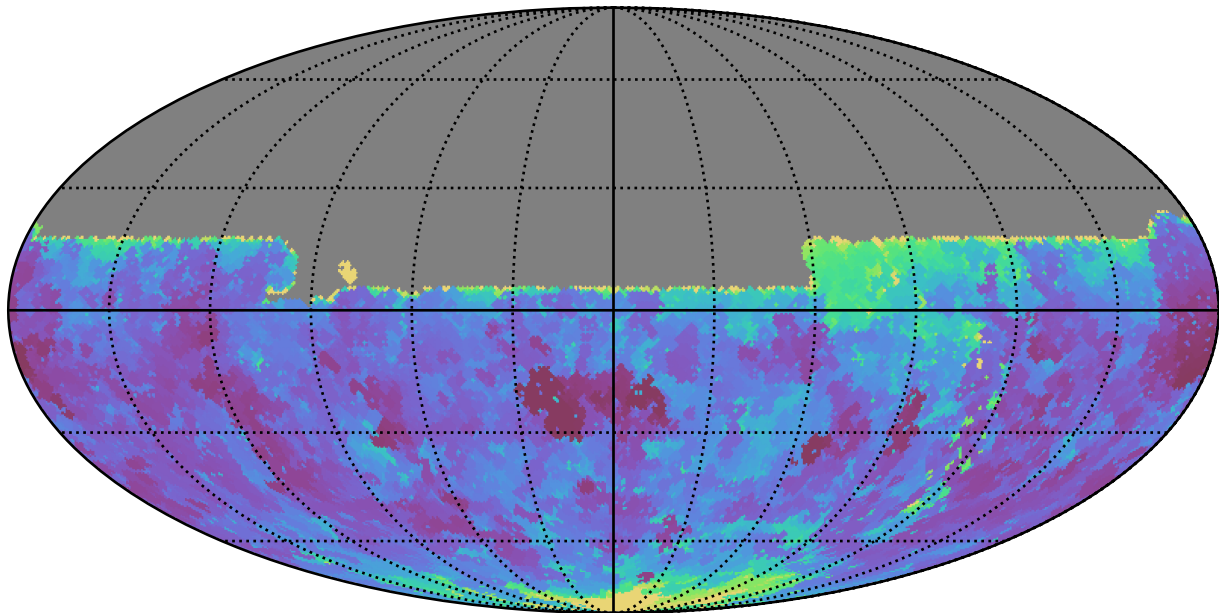
too_combined_s0.8_v3.4_10yrs All sky u band: Min seeingEff
