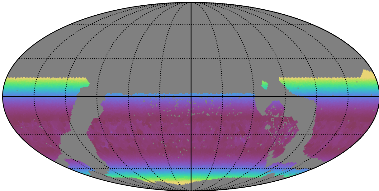
too_combined_s0.8_v3.4_10yrs WFD g band: Min airmass
