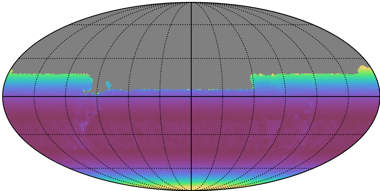
too_combined_s0.8_v3.4_10yrs All sky u band: Min airmass
