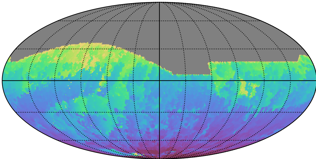
too_combined_s0.8_v3.4_10yrs All sky z band: Min HA
