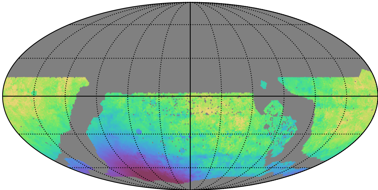
too_combined_s0.8_v3.4_10yrs WFD z band: Median solarElong
