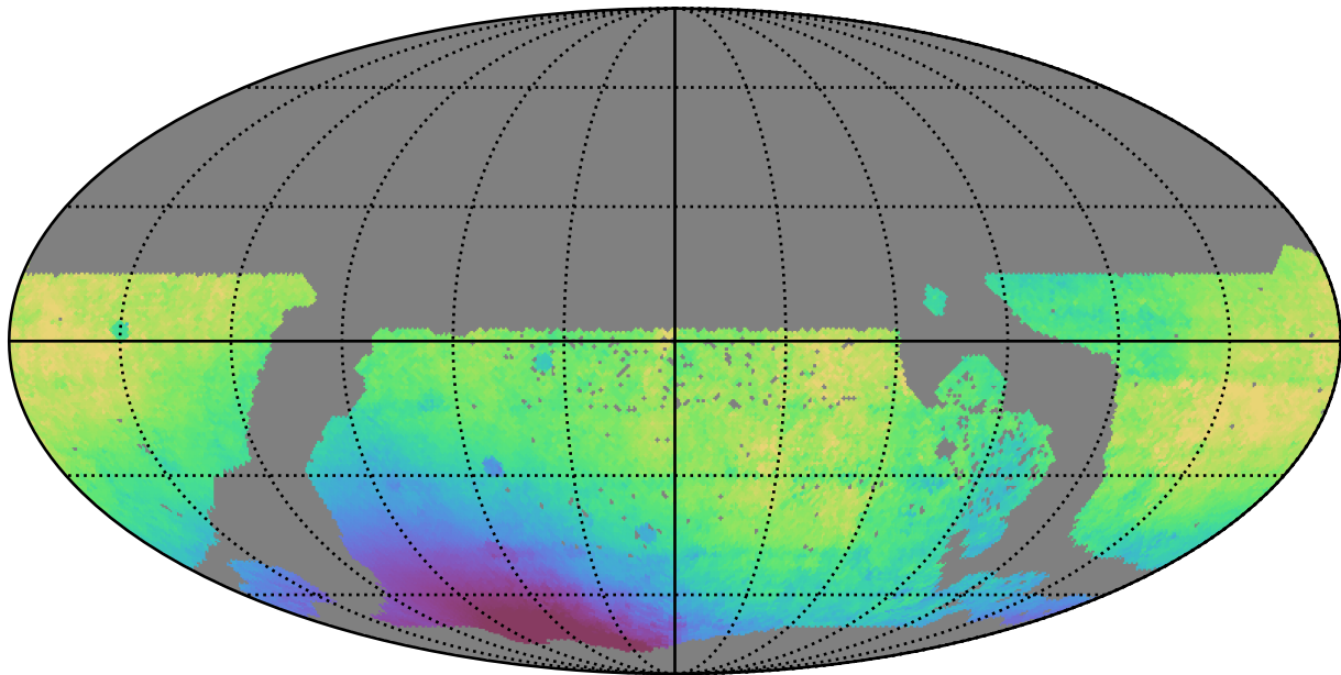
too_combined_s0.8_v3.4_10yrs WFD r band: Median solarElong
