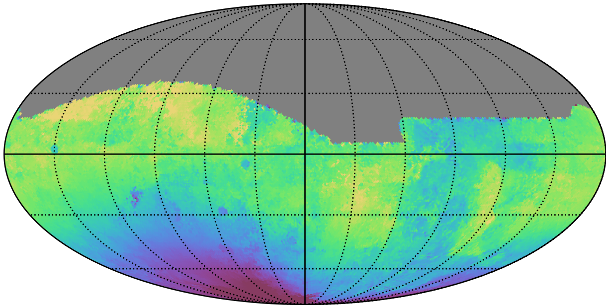
too_combined_s0.8_v3.4_10yrs All sky g band: Median solarElong
