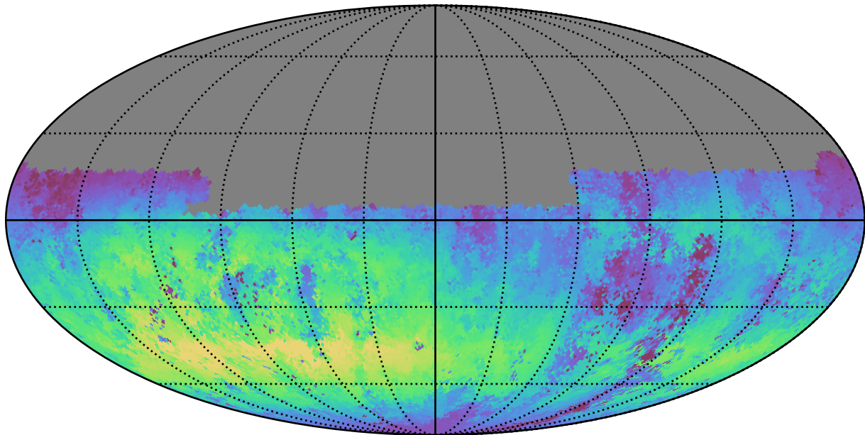
too_combined_s0.8_v3.4_10yrs Yr 1 u band: Median skyBrightness
