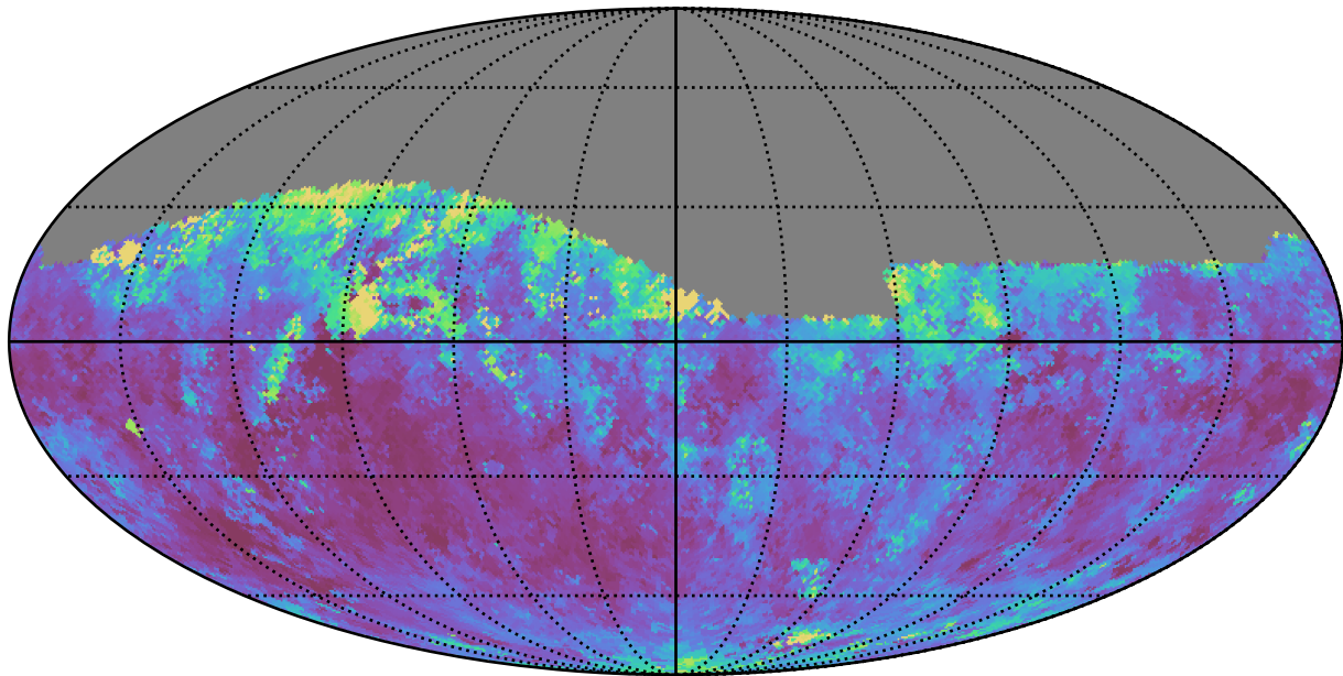
too_combined_s0.8_v3.4_10yrs Yr 1 z band: Median seeingGeom
