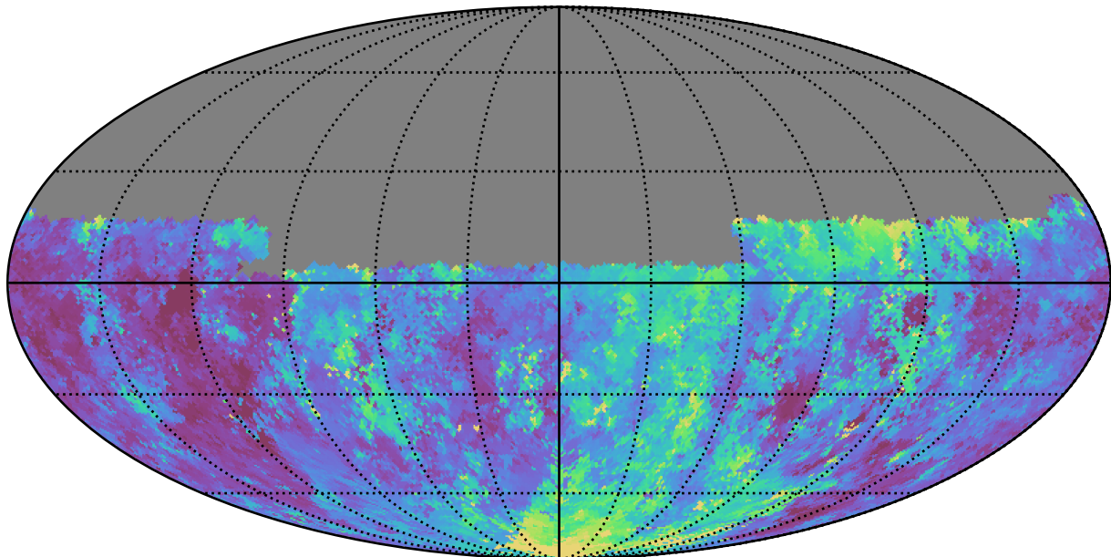
too_combined_s0.8_v3.4_10yrs Yr 1 u band: Median seeingGeom
