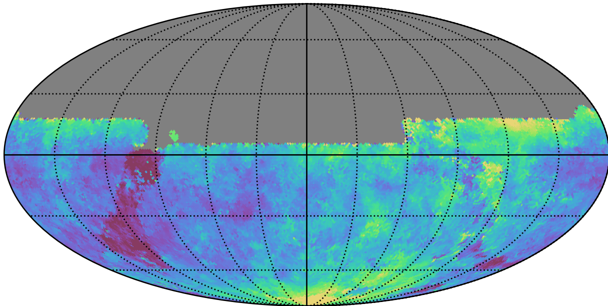
too_combined_s0.8_v3.4_10yrs All sky u band: Median seeingEff
