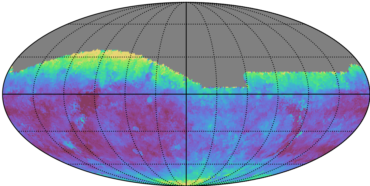
too_combined_s0.8_v3.4_10yrs All sky g band: Median seeingEff
