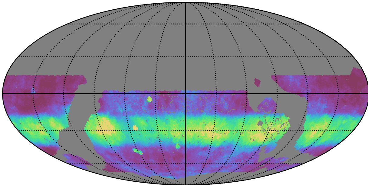
too_combined_s0.8_v3.4_10yrs WFD i band: Median normairmass
