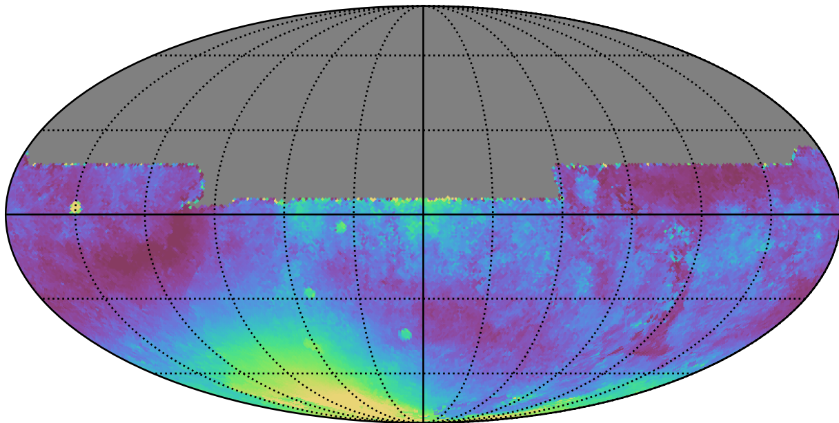
too_combined_s0.8_v3.4_10yrs All sky y band: Median moonDistance
