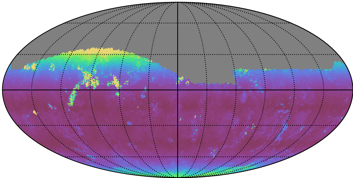
too_combined_s0.8_v3.4_10yrs Yr 1 z band: Median airmass
