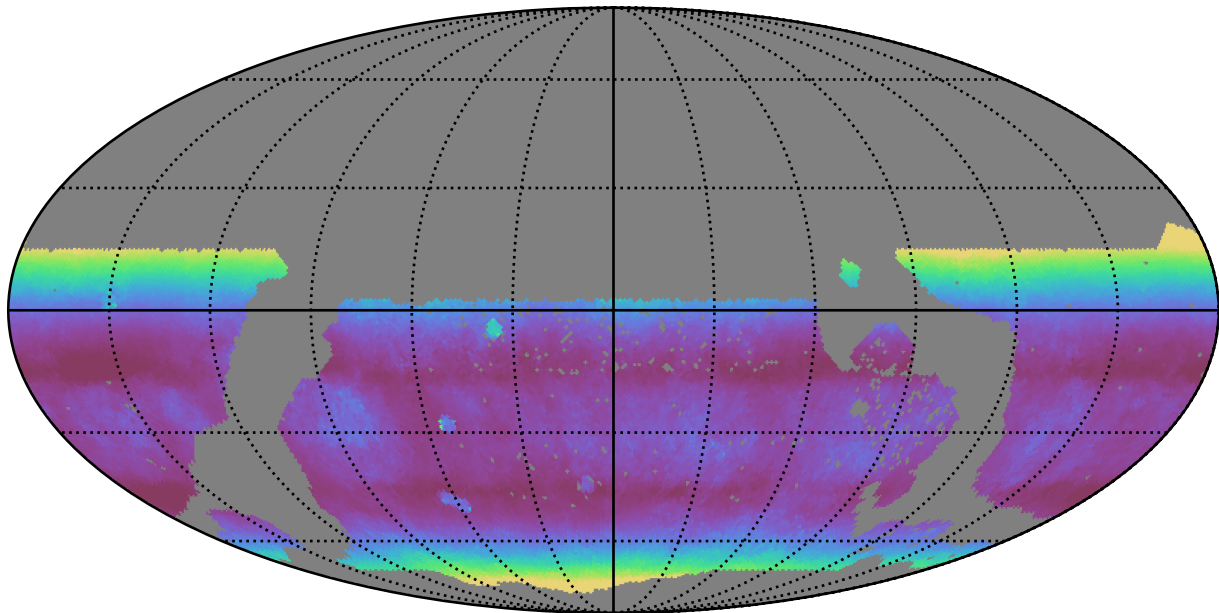
too_combined_s0.8_v3.4_10yrs WFD i band: Median airmass
