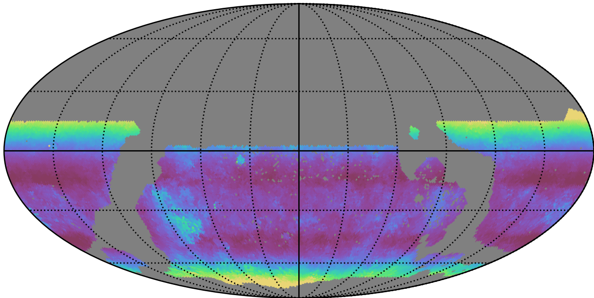
too_combined_s0.8_v3.4_10yrs WFD g band: Median airmass
