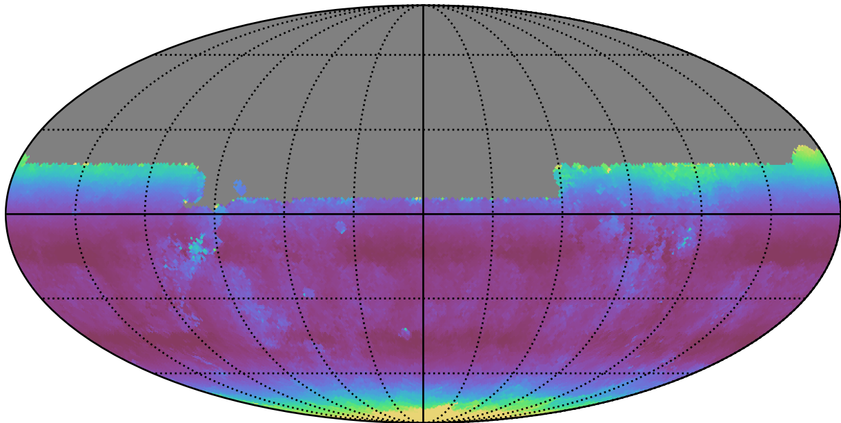
too_combined_s0.8_v3.4_10yrs All sky u band: Median airmass
