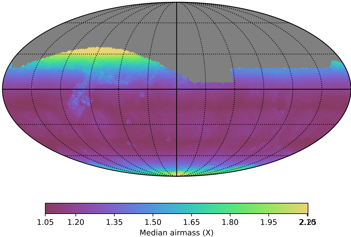
too_combined_s0.8_v3.4_10yrs All sky i band: Median airmass
