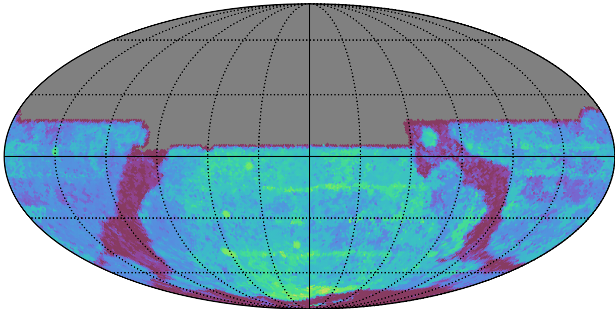
too_combined_s0.8_v3.4_10yrs All sky y band: Median Season Length
