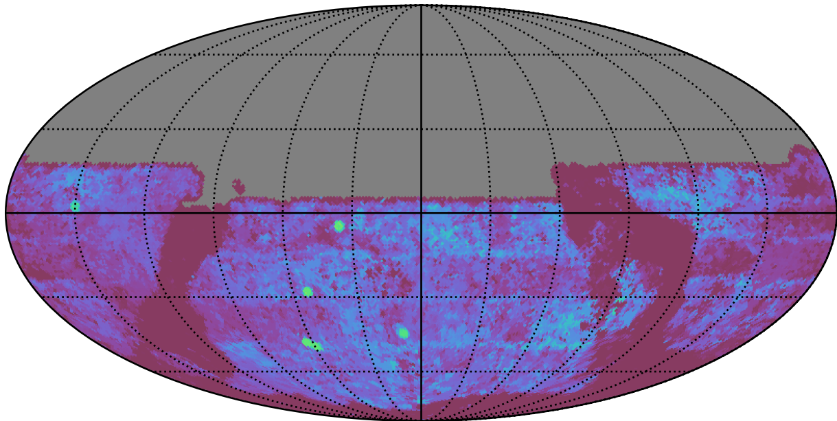
too_combined_s0.8_v3.4_10yrs All sky u band: Median Season Length
