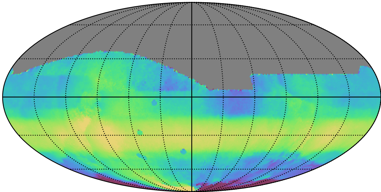
too_combined_s0.8_v3.4_10yrs All sky all bands: Median HA
