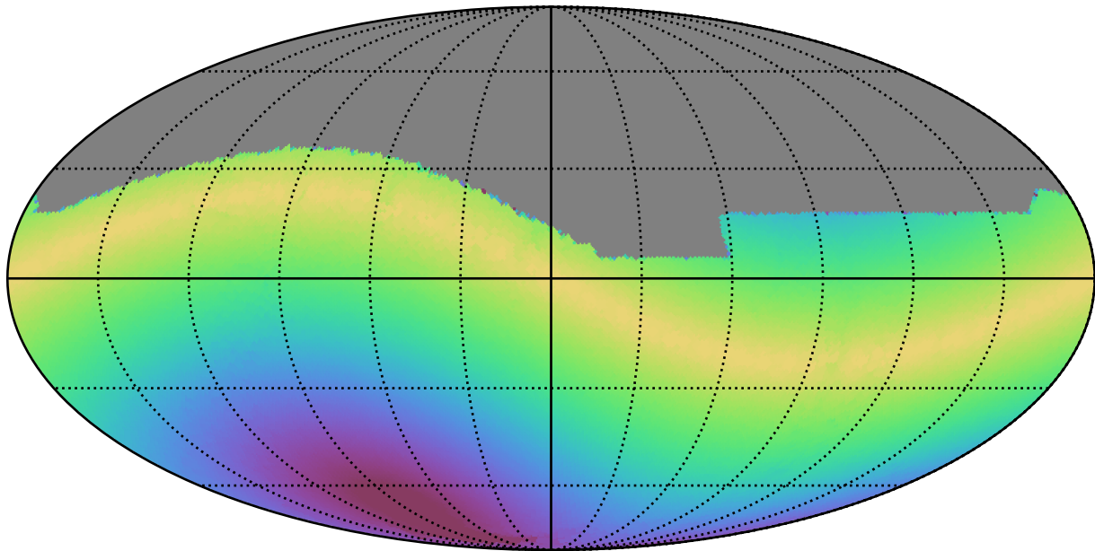
too_combined_s0.8_v3.4_10yrs All sky r band: Max solarElong
