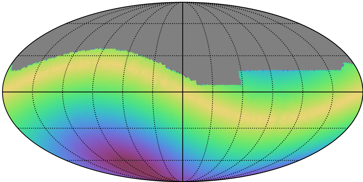
too_combined_s0.8_v3.4_10yrs All sky i band: Max solarElong
