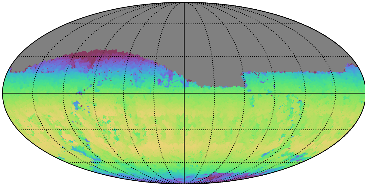
too_combined_s0.8_v3.4_10yrs Yr 1 z band: Max skyBrightness
