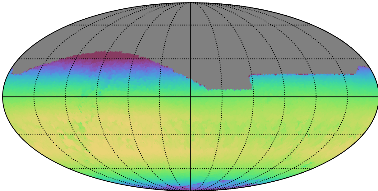
too_combined_s0.8_v3.4_10yrs All sky z band: Max skyBrightness
