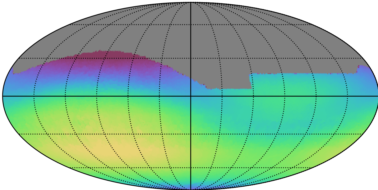
too_combined_s0.8_v3.4_10yrs All sky r band: Max skyBrightness
