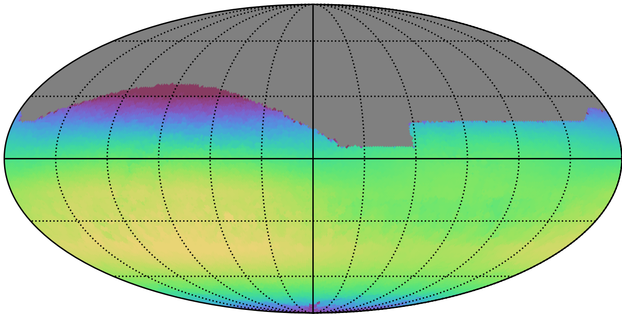
too_combined_s0.8_v3.4_10yrs All sky i band: Max skyBrightness
