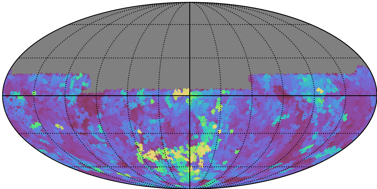
too_combined_s0.8_v3.4_10yrs Yr 1 y band: Max seeingEff
