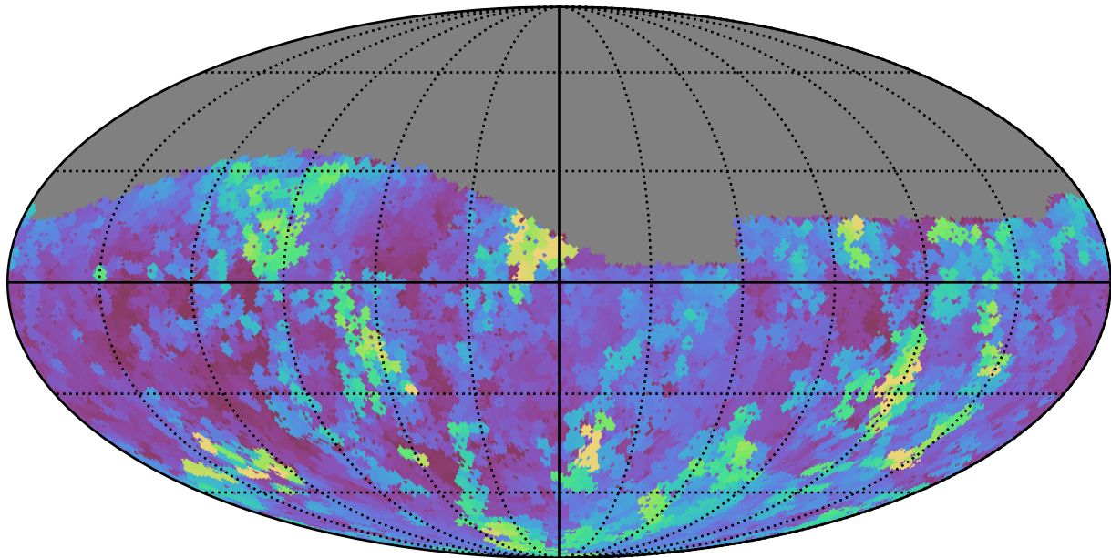
too_combined_s0.8_v3.4_10yrs Yr 1 g band: Max seeingEff
