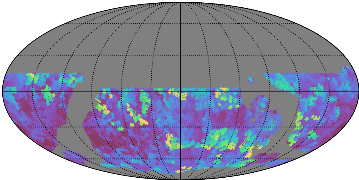
too_combined_s0.8_v3.4_10yrs WFD i band: Max seeingEff
