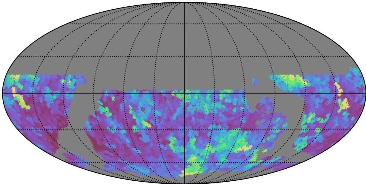
too_combined_s0.8_v3.4_10yrs WFD all bands: Max seeingEff
