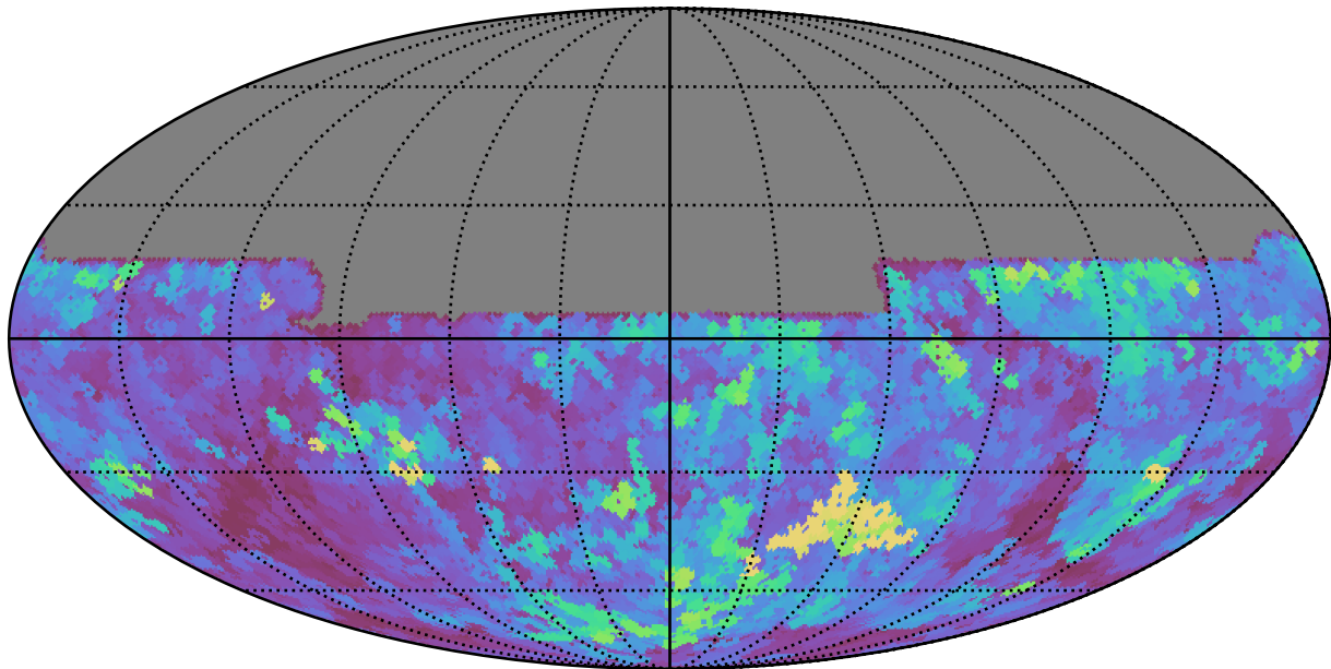
too_combined_s0.8_v3.4_10yrs All sky y band: Max seeingEff
