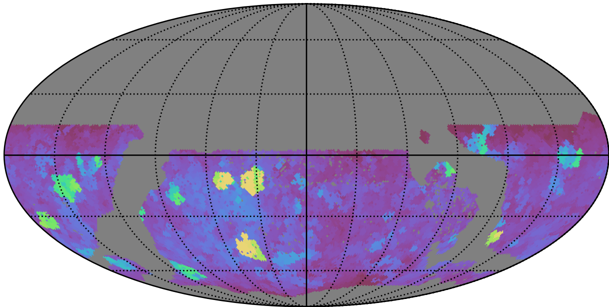
too_combined_s0.8_v3.4_10yrs WFD i band: Max saturation_mag
