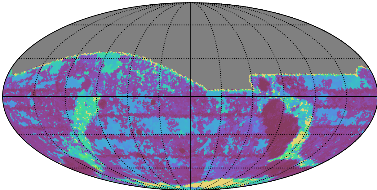
too_combined_s0.8_v3.4_10yrs All sky g band: Max Inter-Night Gap
