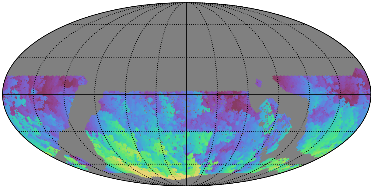
too_combined_s0.8_v3.4_10yrs WFD u band: Max HA
