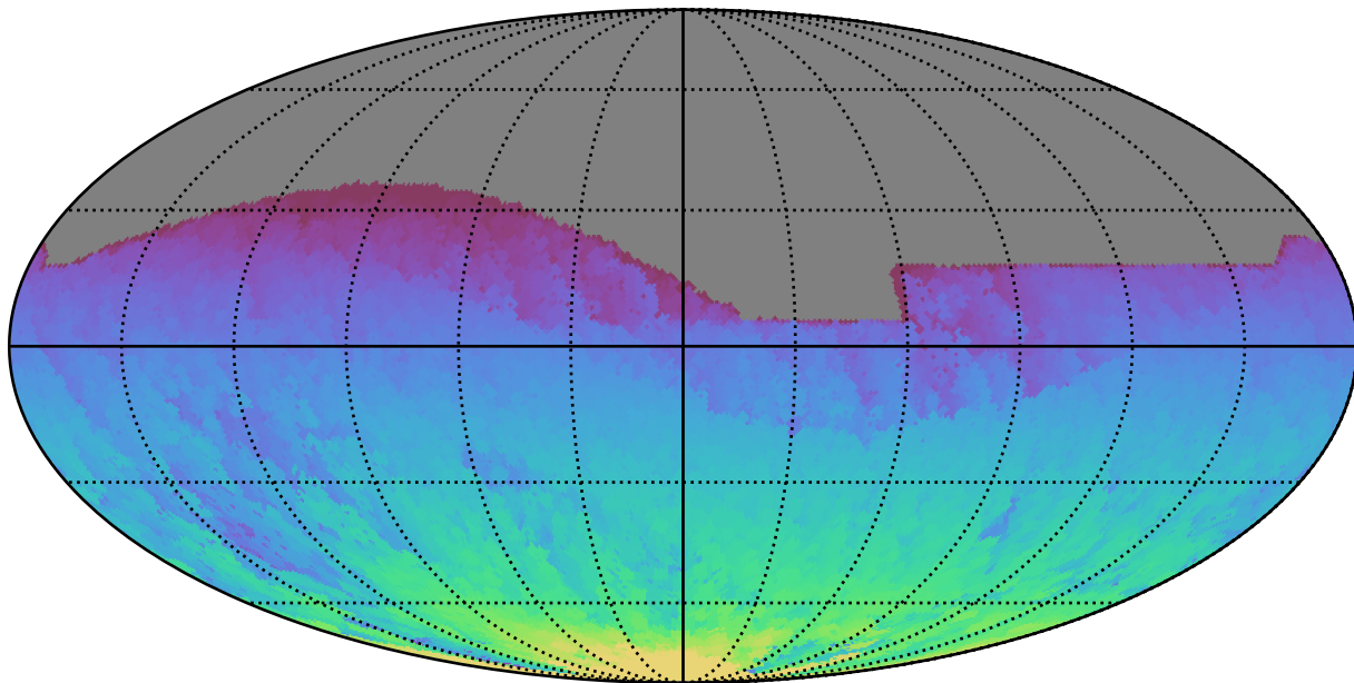
too_combined_s0.8_v3.4_10yrs All sky all bands: Max HA
