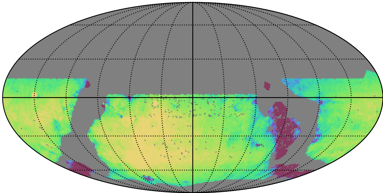
too_combined_s0.8_v3.4_10yrs WFD r band: Exgal_CoaddM5
