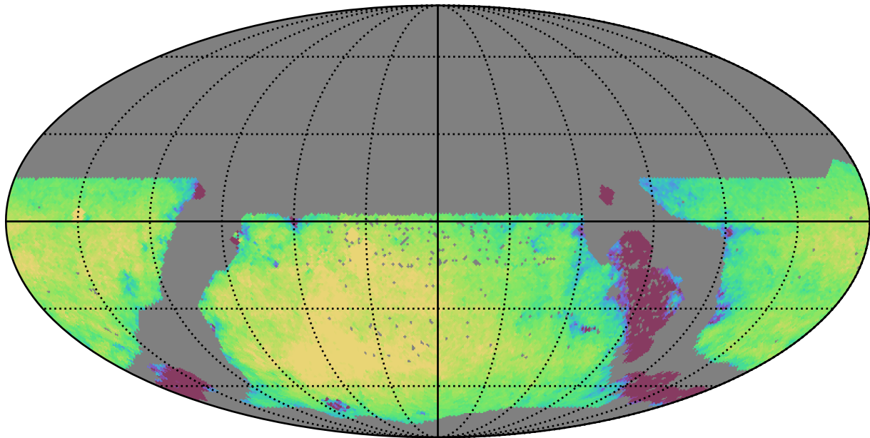
too_combined_s0.8_v3.4_10yrs WFD g band: Exgal_CoaddM5
