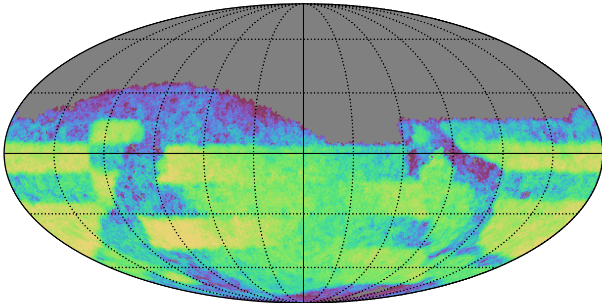
too_combined_s0.8_v3.4_10yrs Yr 3-4 z band: CoaddM5
