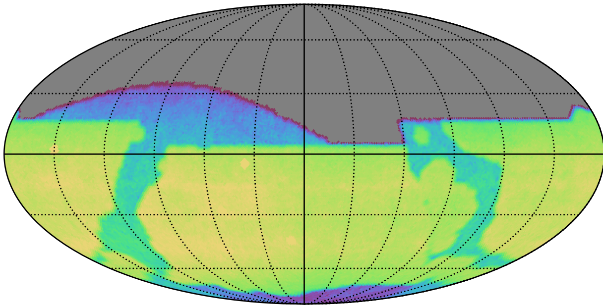
too_combined_s0.8_v3.4_10yrs All sky z band: CoaddM5
