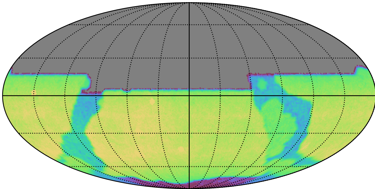
too_combined_s0.8_v3.4_10yrs All sky y band: CoaddM5
