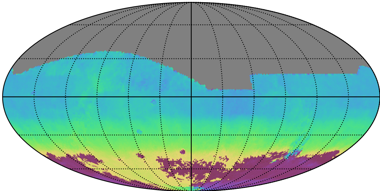
too_combined_s0.8_v3.4_10yrs All sky i band: AngleMean rotSkyPos
